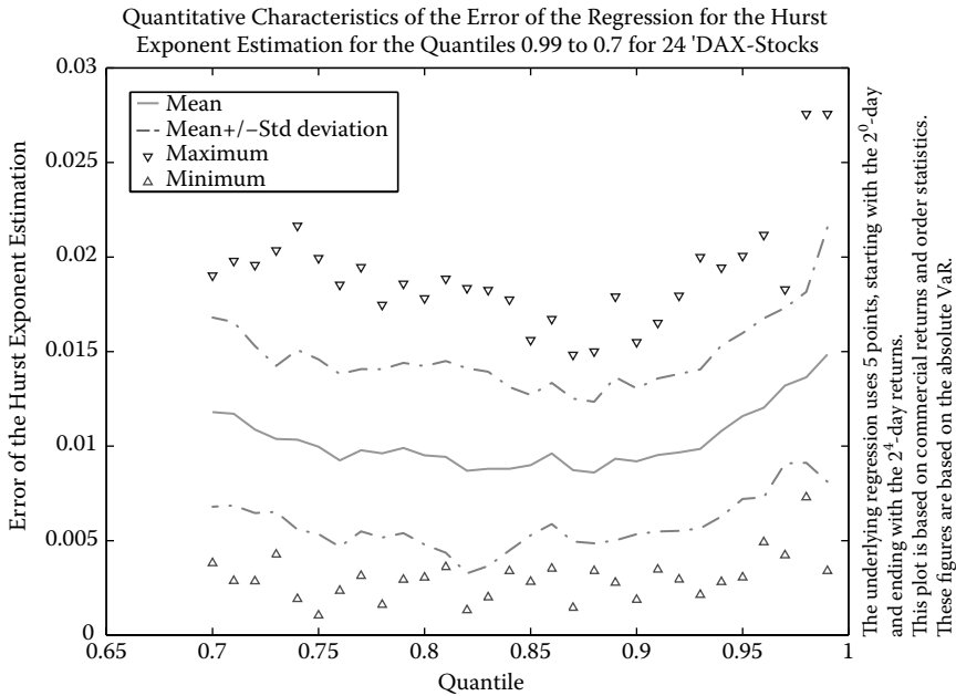
The solid line is the mean, the dash-dotted lines are the mean plus/minus the standard deviation, the triangles are the minimum, and the upside down triangles are the maximum of the error curves of the estimation for the scaling law, which are based on 24 DAX-stocks. The underlying time series is a commercial return. Shown are the lower (left) quantiles (see Figure 13.6.4) and the upper (right) quantiles (see Figure 13.6.5).
